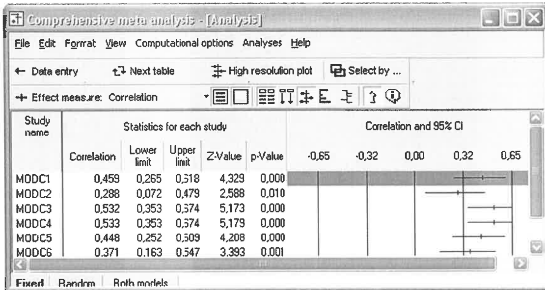
Fig. 6. Time vs. MOD SubComp meta-analysis (hypothesis 4).
