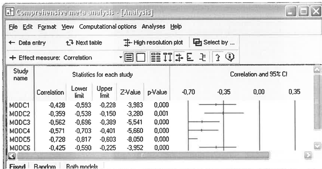
Fig. 7. Efficiency vs. MOD SubComp meta-analysis (hypothesis 5).
