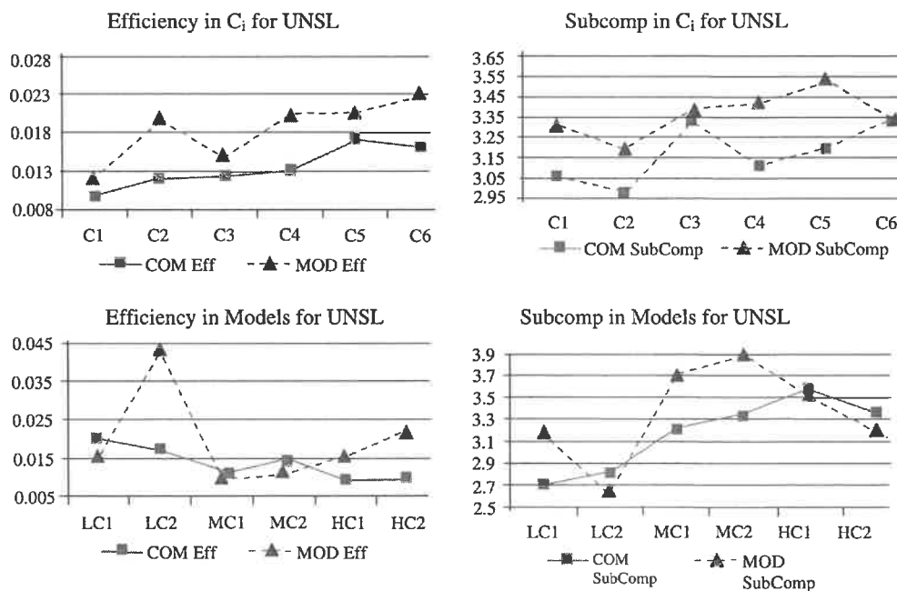
Fig. 5. Descriptive statistics for UNSL.
