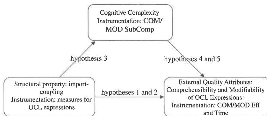
Fig. 3. Experimental hypotheses.
