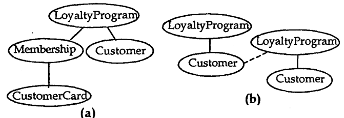
Fig. 3: Examples of navigation trees
